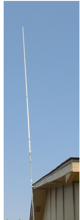
Figure 53 - Buddi Pole HF dipole above and 440 MHz vertical on the right. Photos by K3DIO
