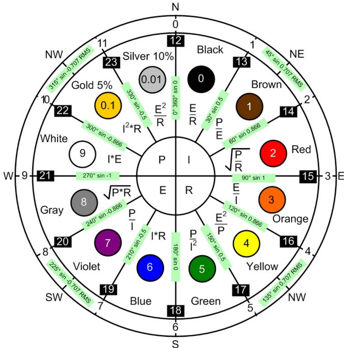
Figure 64 - Ohms Law Summary artwork. N5IUT
